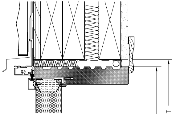
HEAD DETAIL 2x6 STUD WALL
