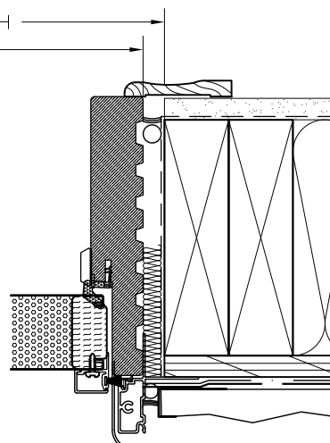
SILL DETAIL 2x4 STUD WALL
