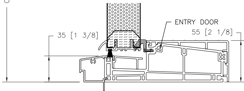
SAMPLE ELEVATION EXTERIOR VIEW
