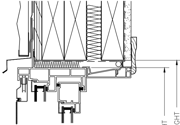
HEAD DETAIL 2x6 STUD WALL
