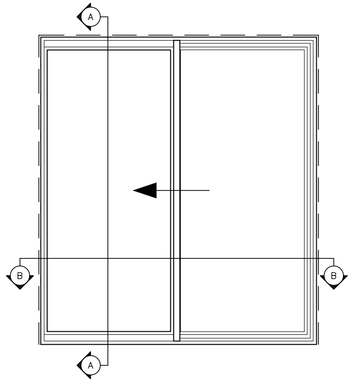
SAMPLE ELEVATION EXTERIOR VIEW
