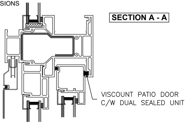
HEAD DETAIL FRAME DIMENSIONS
