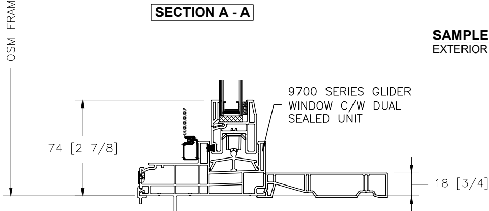
SILL DETAIL FRAME DIMENSIONS
