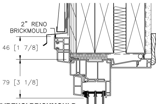
B - 2" 'RENO' BRICKMOULD
