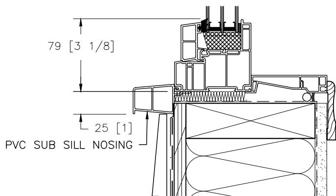
C - PVC SUBSILL NOSING
