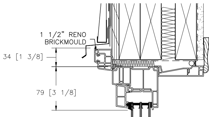
A - 1 1/2" RENO BRICKMOULD
