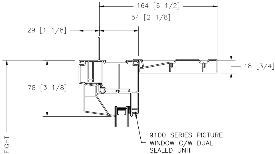
HEAD DETAIL FRAME DIMENSIONS
