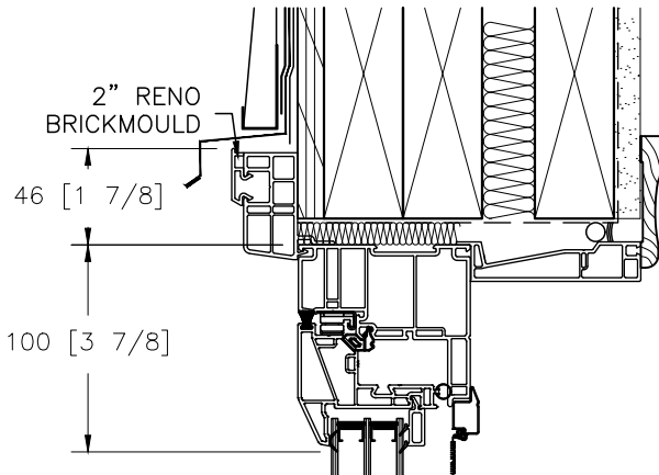
B - 2" 'RENO' BRICKMOULD
