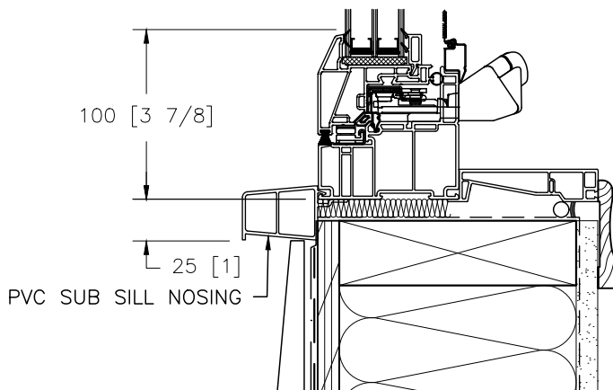
C - PVC SUBSILL NOSING
