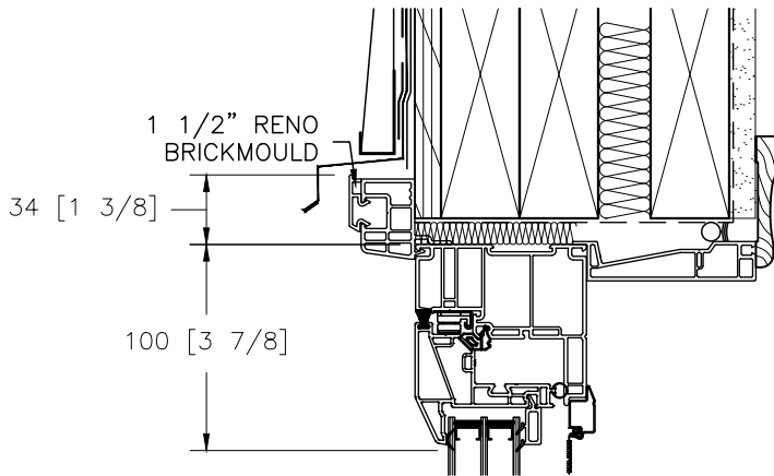
A - 1 1/2" RENO BRICKMOULD
