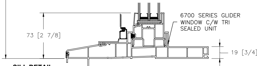
SILL DETAIL TRIPANE WITH 7 1/2" JAMB
