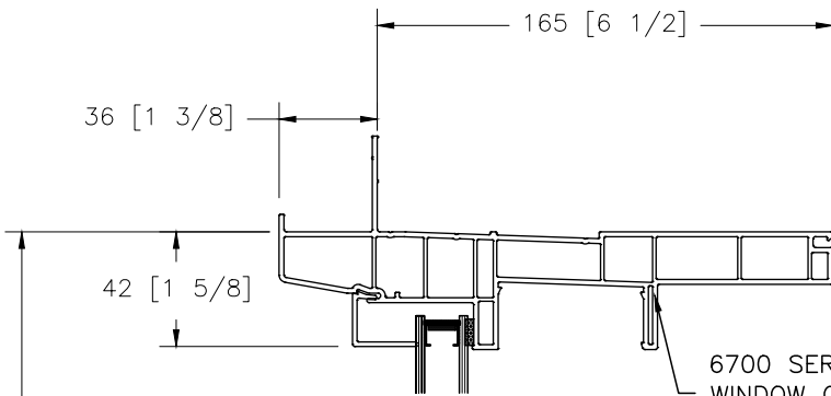
HEAD DETAIL FRAME DIMENSIONS
