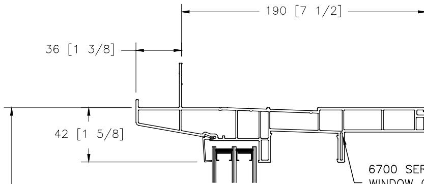
HEAD DETAIL TRIPANE WITH 7 1/2" JAMB
