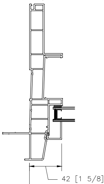
SILL DETAIL FRAME DIMENSIONS
