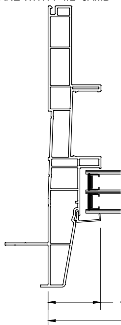
JAMB DETAIL TRIPANE WITH 7 1/2" JAMB
