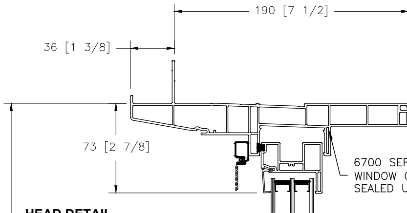
HEAD DETAIL TRIPANE WITH 7 1/2" JAMB
