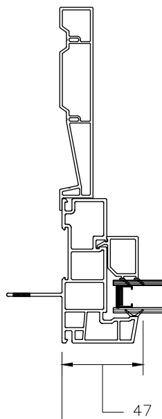
SILL DETAIL FRAME DIMENSIONS
