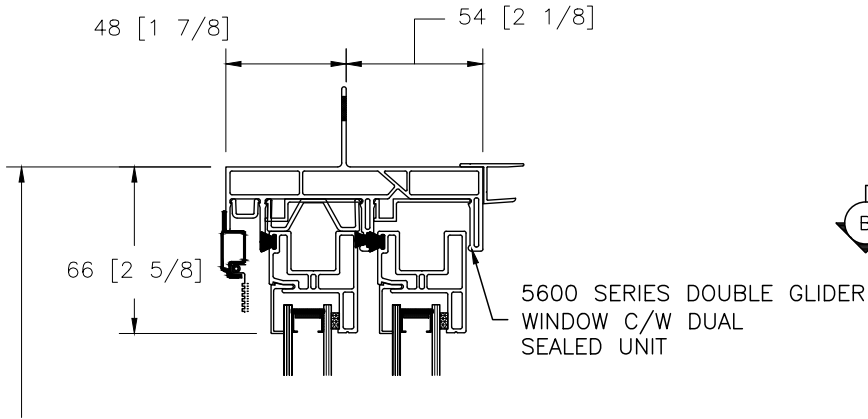
HEAD DETAIL FRAME DIMENSIONS
