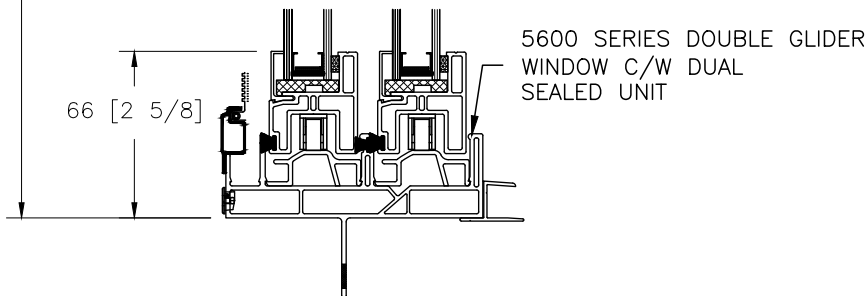
SILL DETAIL FRAME DIMENSIONS
