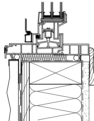
SILL DETAIL 2x4 STUD WALL
