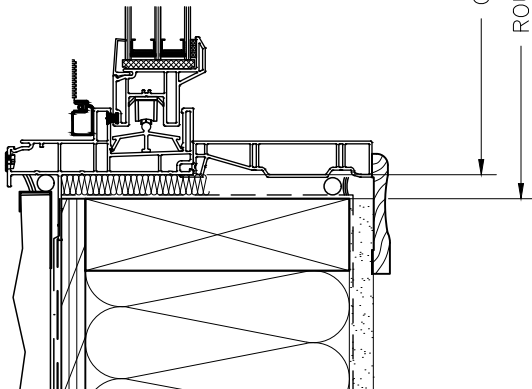
SILL DETAIL 2x4 STUD WALL
