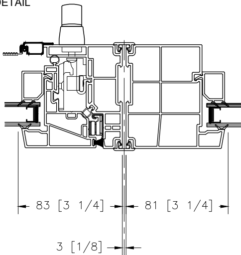
C. AWNING - FIXED MULLION DETAIL
