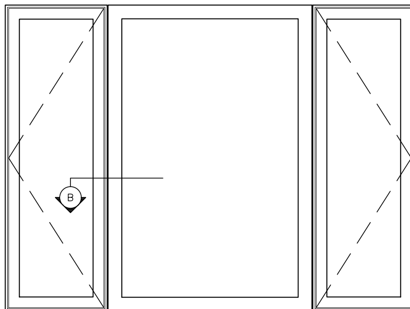
SAMPLE ELEVATION EXTERIOR VIEW
