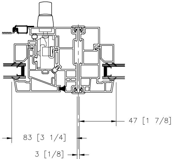
A. PICTURE - PICTURE MULLION DETAIL
