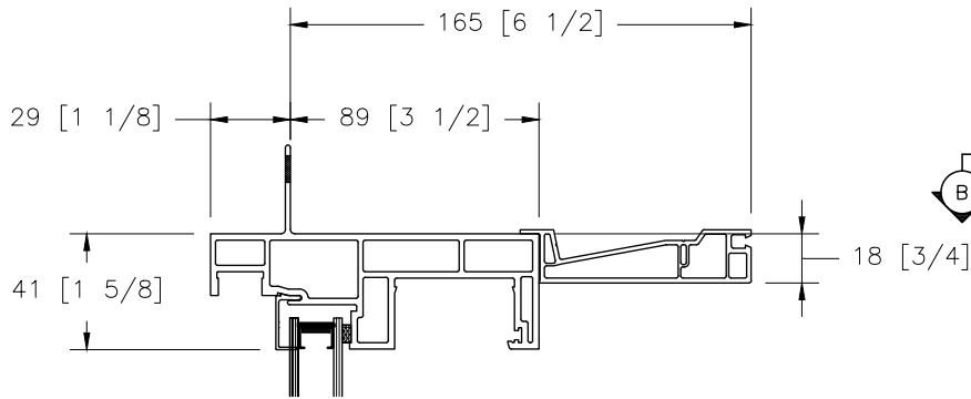
HEAD DETAIL FRAME DIMENSIONS
