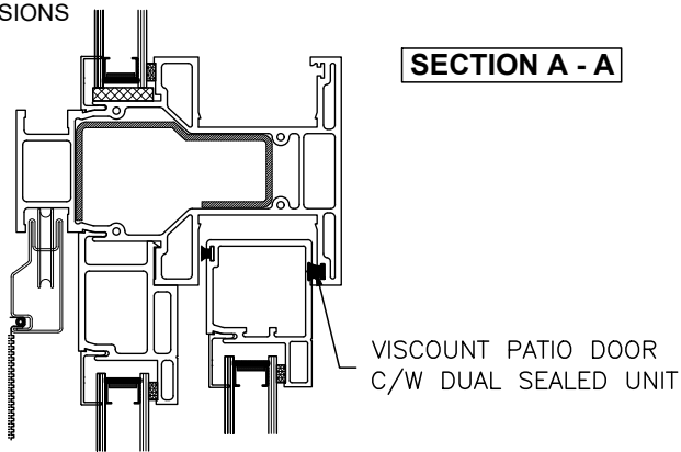
MULLION DETAIL FRAME DIMENSIONS
