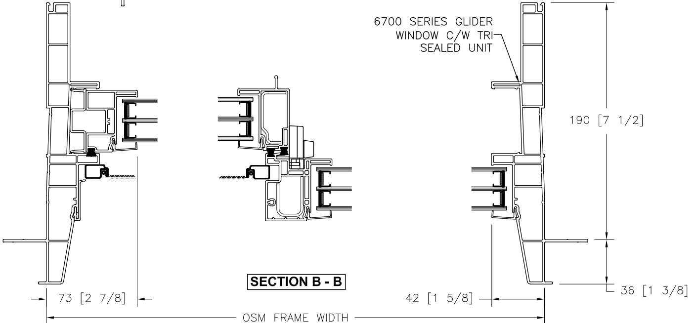
JAMB DETAIL TRIPANE WITH 7 1/2" JAMB
