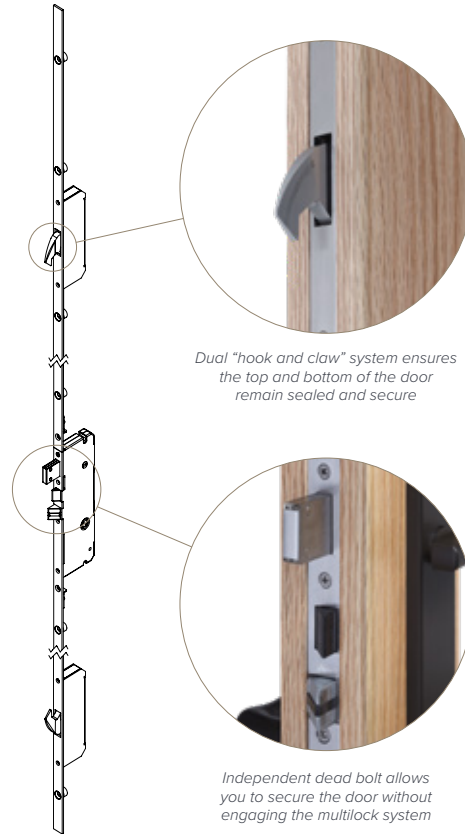
3-Point "Hook & Claw" Multilock Assembly
