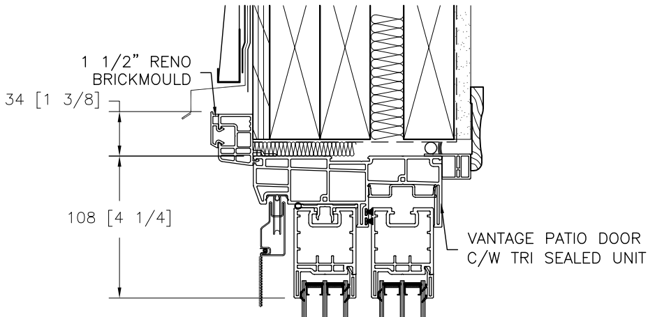
B - 1 1/2" 'RENO' BRICKMOULD OPTION
