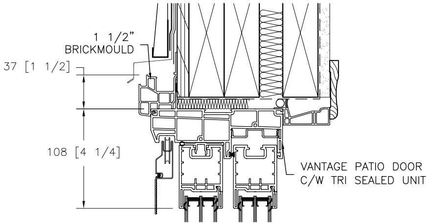
A - 1 1/2" BRICKMOULD OPTION
