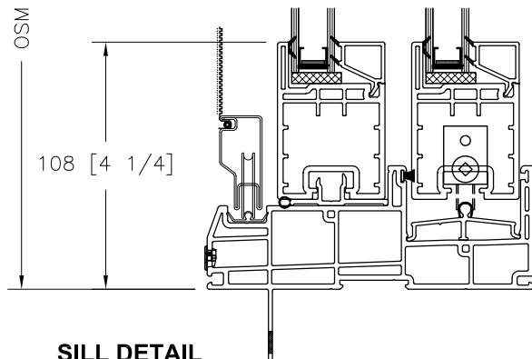
SILL DETAIL FRAME DIMENSIONS
