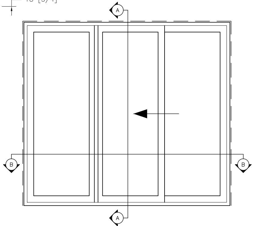
SAMPLE ELEVATION EXTERIOR VIEW
