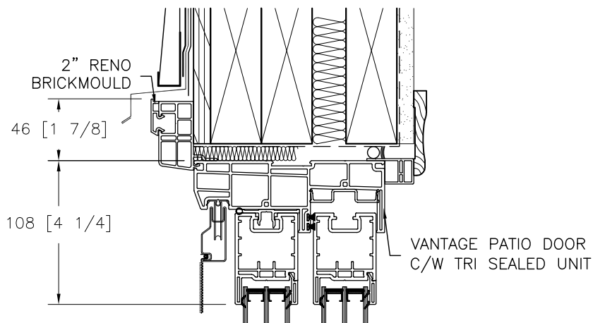
C - 2" 'RENO' BRICKMOULD OPTION
