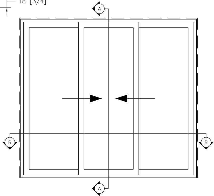
SAMPLE ELEVATION EXTERIOR VIEW
