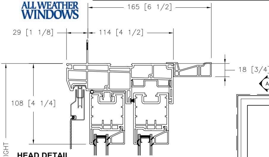
HEAD DETAIL FRAME DIMENSIONS
